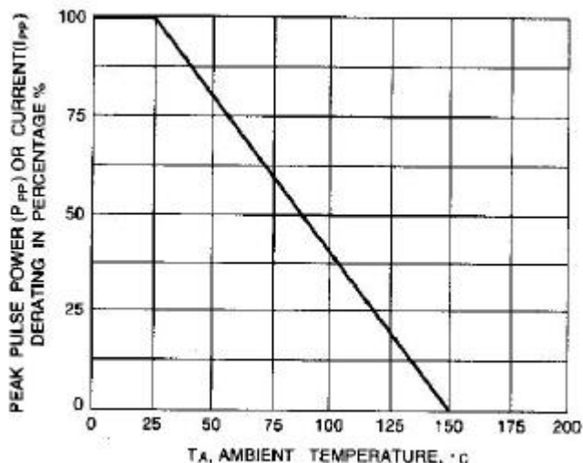
Fig. 2-PULSE RATING CURVE
