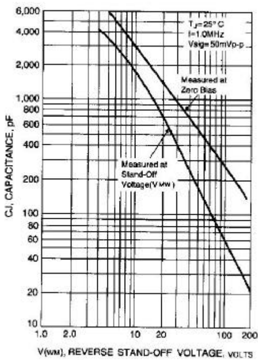
Fig. 4-TYPICAL JUNCTION
