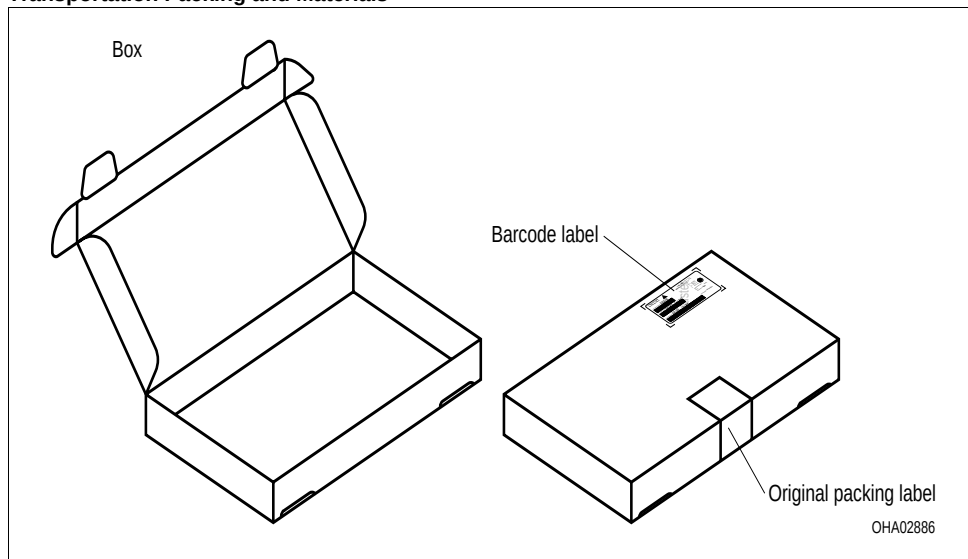
Dimensions of transportation box in mm (inch)
