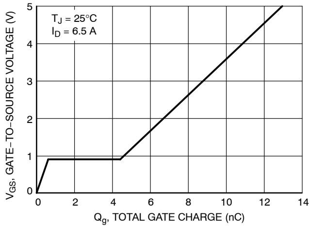
Figure 7. Gate-to-Source
