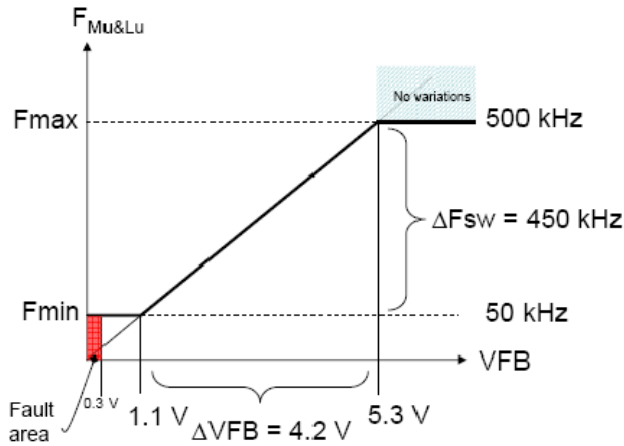
Figure 27. Maximal Default Excursion, R t = 34 kΩ on Pin 4 and R F(max) = 1.9 kΩ on Pin 2
