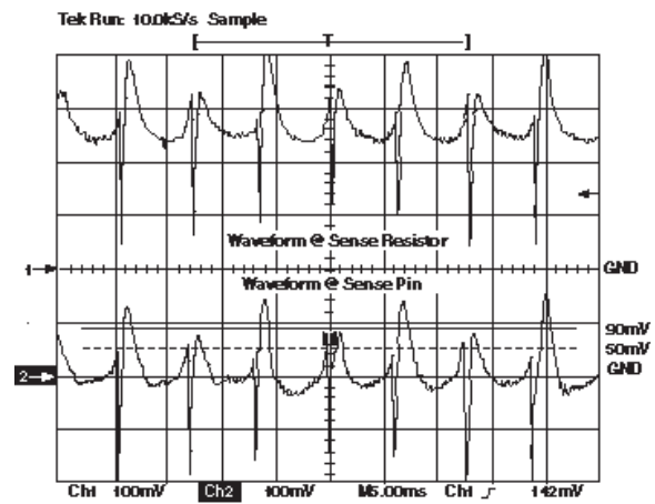
Figure 8. SENSE Waveforms
