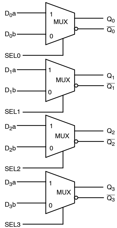
Figure 2. Logic Diagram
