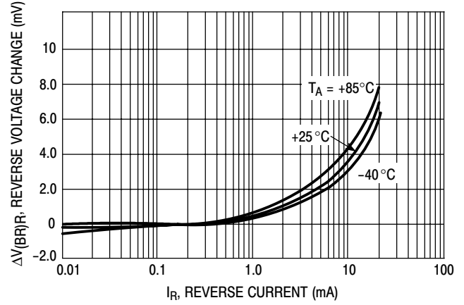
Figure 3. Reverse Characteristics
