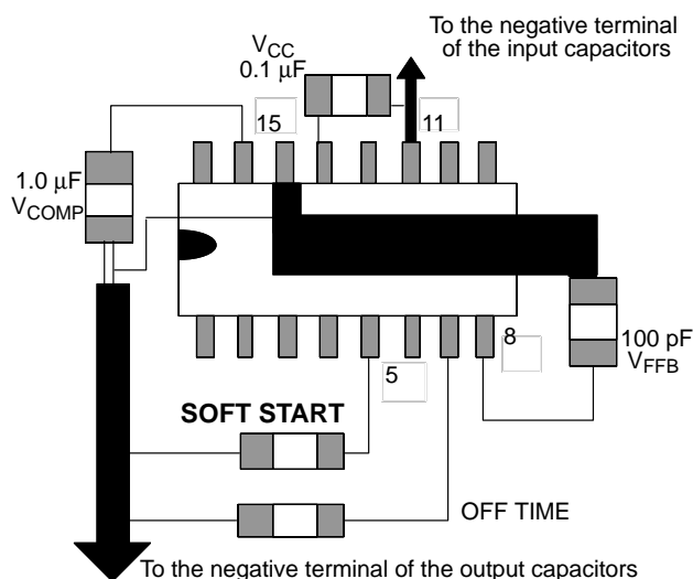
Figure 20. Layout Guidelines
