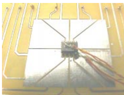
Figure 25. 1.0 oz. copper, approx. 1/8 in 2 per lead, 1.0 in 2 total
