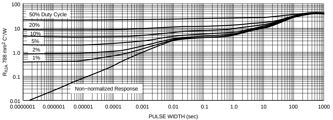
Figure 11. Duty Cycle for 1" Spreaders Boards, D²PAK 5-Lead
