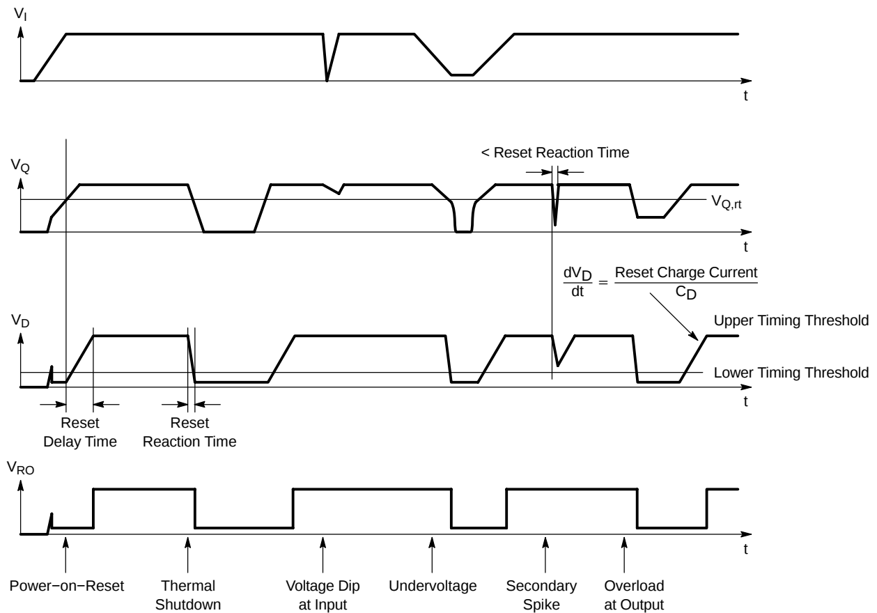
Figure 5. Reset Timing
