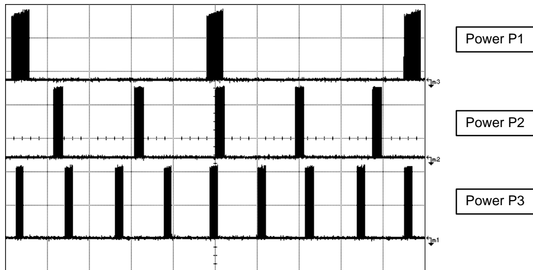
Figure 18. Output Pulses at Various Power Levels ( X = 5.0\text{ μs/div} ) P1 < P2 < P3
