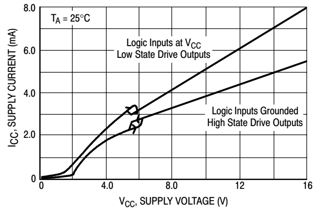
Figure 17. Supply Current versus Supply Voltage
