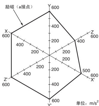
误动作冲击
