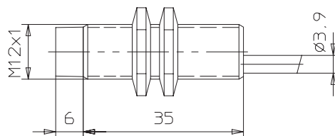
E2EL-X4M□ 2M
