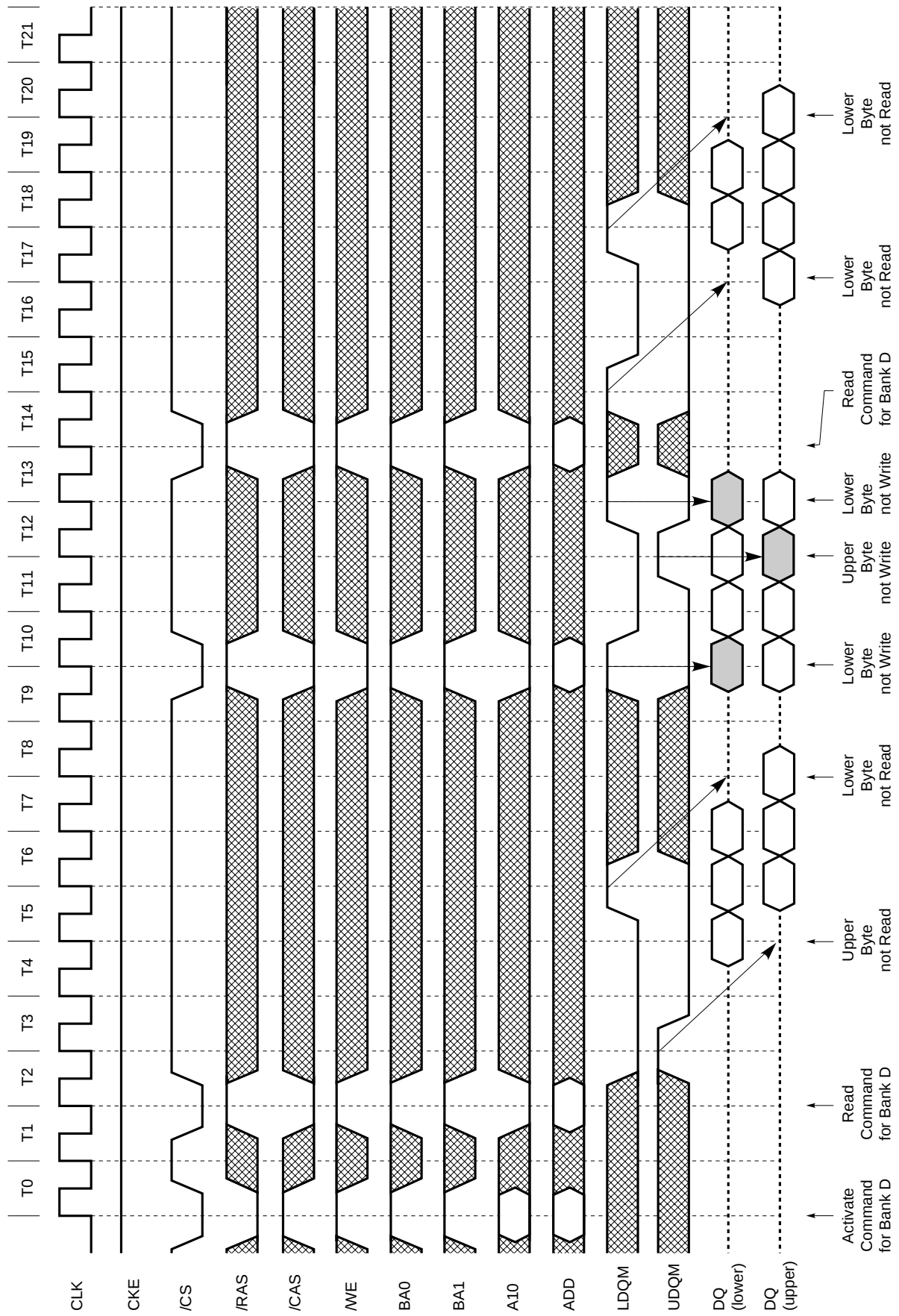
Byte Write Operation (Burst Length = 4, /CAS Latency = 3)
