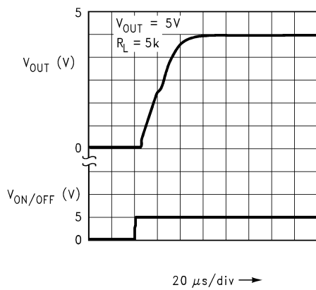
Turn-On Waveform
