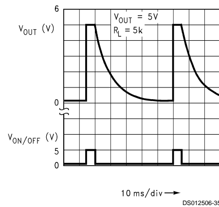
Turn-Off Waveform
