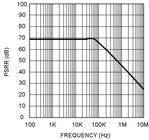
PSRR vs. Frequency @ 5V
