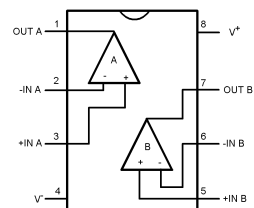
LMH6655 in SOIC and MSOP
