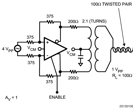
FIGURE 11. Transformer Out Low Impedance Load
