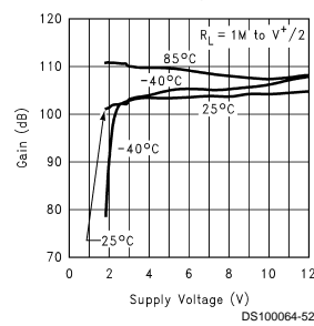
Large Signal Voltage Gain vs Supply Voltage
