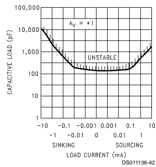
Stability vs Capacitive Load ( A_V = +1 )
