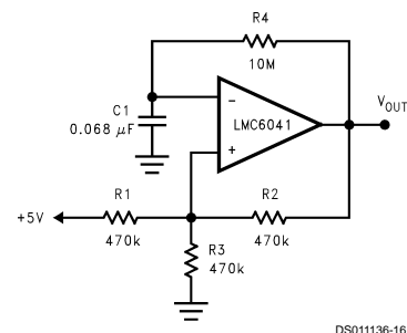
FIGURE 11. 1 Hz Square-Wave Oscillator
