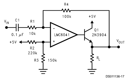
FIGURE 12. AC Coupled Power Amplifier
