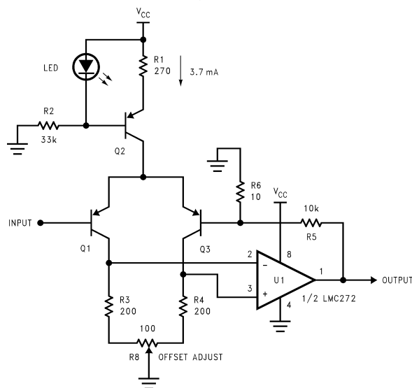
Low Noise Single Supply Preamplifier
