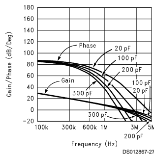
Gain/Phase vs Capacitive Load
