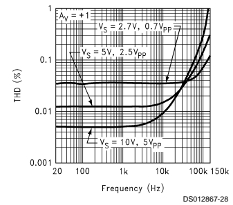
THD vs Frequency
