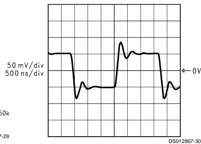
Small Signal Step Response
