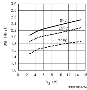
Unity Gain Frequency vs Temperature
