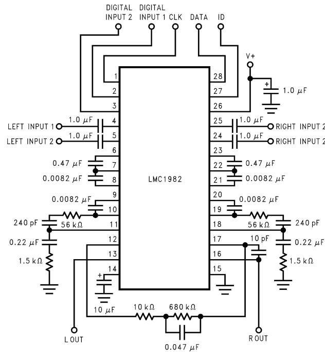
FIGURE 1. Typical Application
