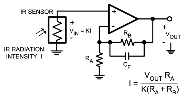
FIGURE 17. IR Radiation Sensor
