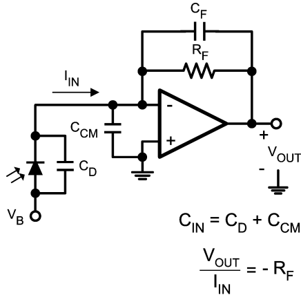
FIGURE 13. Photodiode Transimpedance Amplifier
