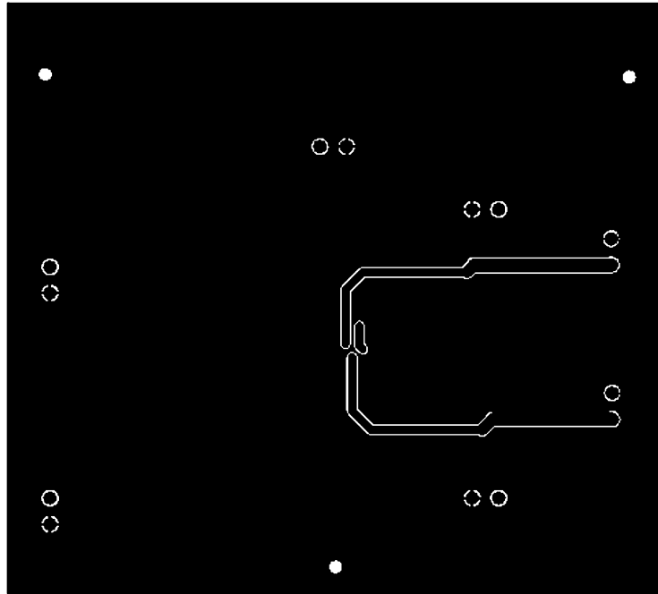
Recommended LLP Board Layout: Bottom Layer
