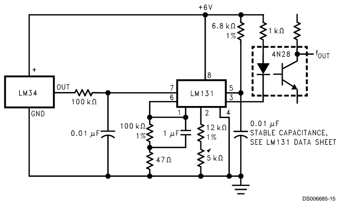
LM34 with Voltage-to-Frequency Converter and Isolated Output (3°F to + 300°F; 30 Hz to 3000 Hz)
