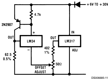
4-to-20 mA Current Source (0 to +100°F)
