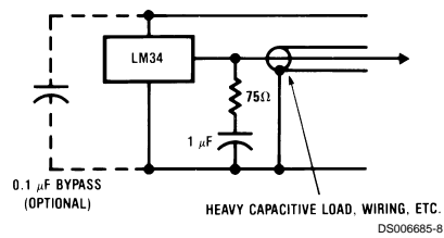
FIGURE 4. LM34 with R-C Damper
