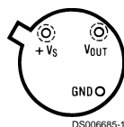
TO-46 Metal Can Package (Note 1)
