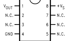
SO-8 Small Outline Molded Package
