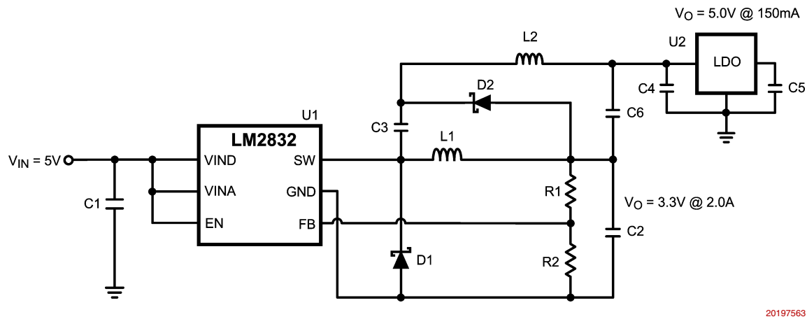
FIGURE 14. LM2832X (1.6MHz): V_{in} = 5V , V_o = 3.3V @ 2.0A & LP2986-5.0 @ 150mA
