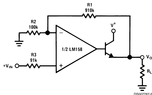
Power Amplifier
