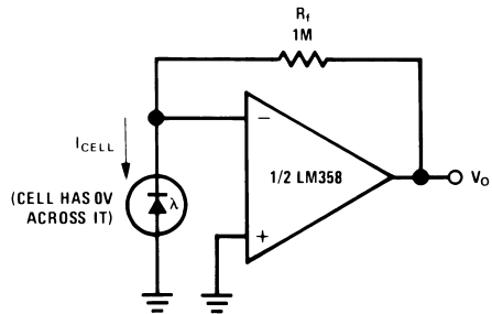
Photo Voltaic-Cell Amplifier
