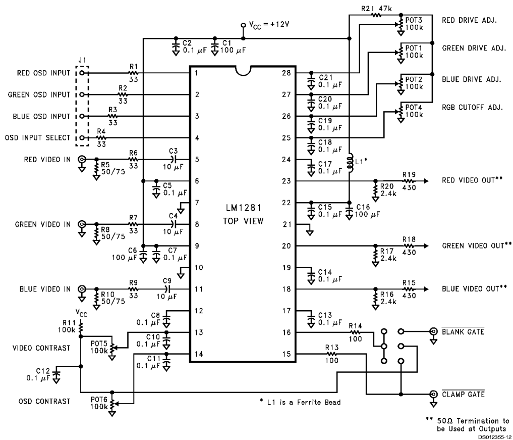
FIGURE 7. LM1281 OSD Video Preamp Demonstration Board Schematic
