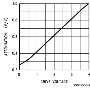
Attenuation vs Drive Voltage
