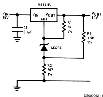
High Stability 10V Regulator
