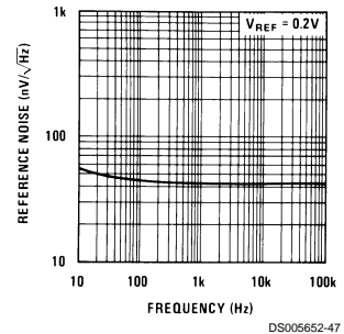
Reference Noise Voltage
