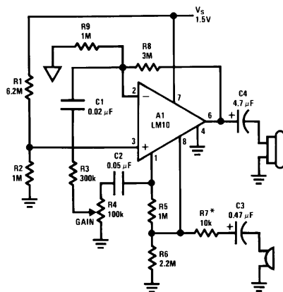
Microphone Amplifier
