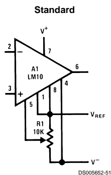
Op Amp Offset Adjustment
