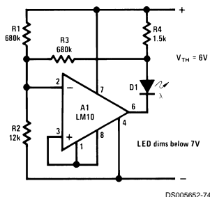
Battery-level Indicator
