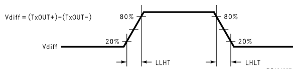
FIGURE 2. DS90CR287 (Transmitter) LVDS Output Load and Transition Times
