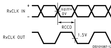
FIGURE 9. DS90CR288A (Receiver) Clock In to Clock Out Delay
