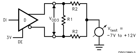
FIGURE 5. V_{OD3}
