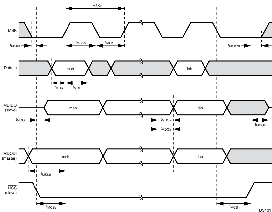
Figure 66. Microwire Transaction Timing, Normal Mode, SCIDL = 0
