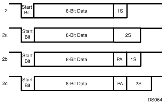
Figure 28. 8-Bit Data Frame Options
