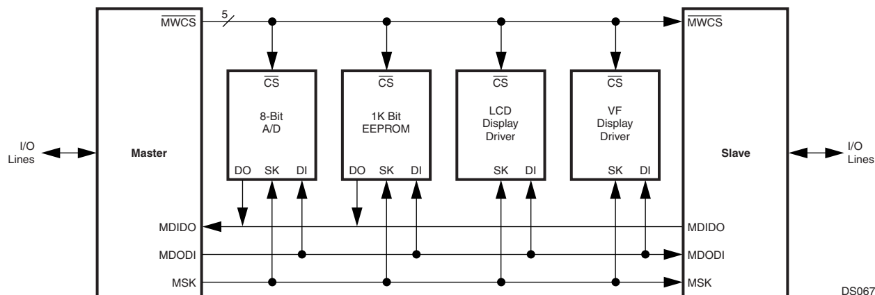
Figure 31. Microwire Interface
