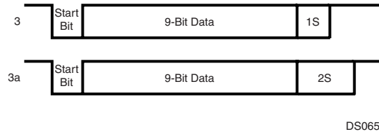
Figure 29. 9-bit Data Frame Options
