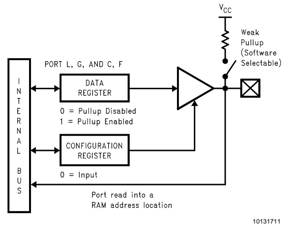
FIGURE 6. I/O Port Configurations—Input Mode
