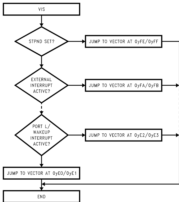
FIGURE 27. VIS Flowchart
