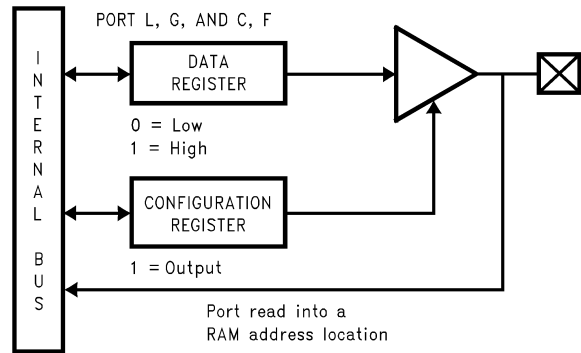
FIGURE 5. I/O Port Configurations—Output Mode
