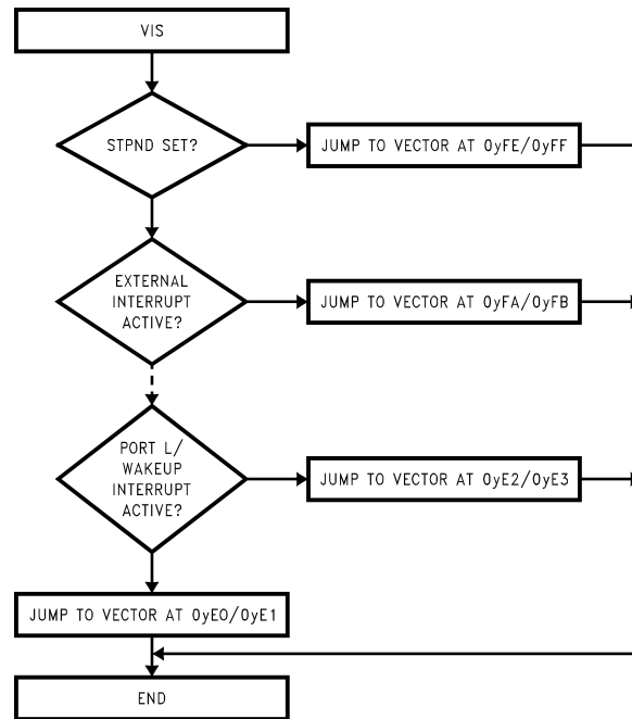
FIGURE 28. VIS Flowchart
