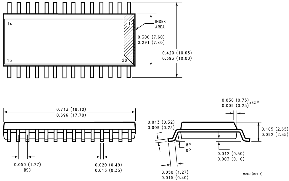
Molded SO Wide Body Package (WM) Order Number COP8FGx528Mx, NS Package Number M28B
