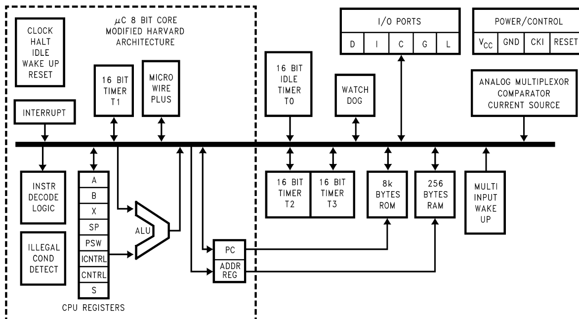
FIGURE 1. Block Diagram
