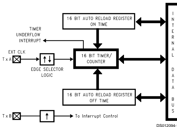
FIGURE 9. Timer in External Event Counter Mode
