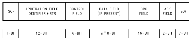
FIGURE 21. CAN Frame Format
