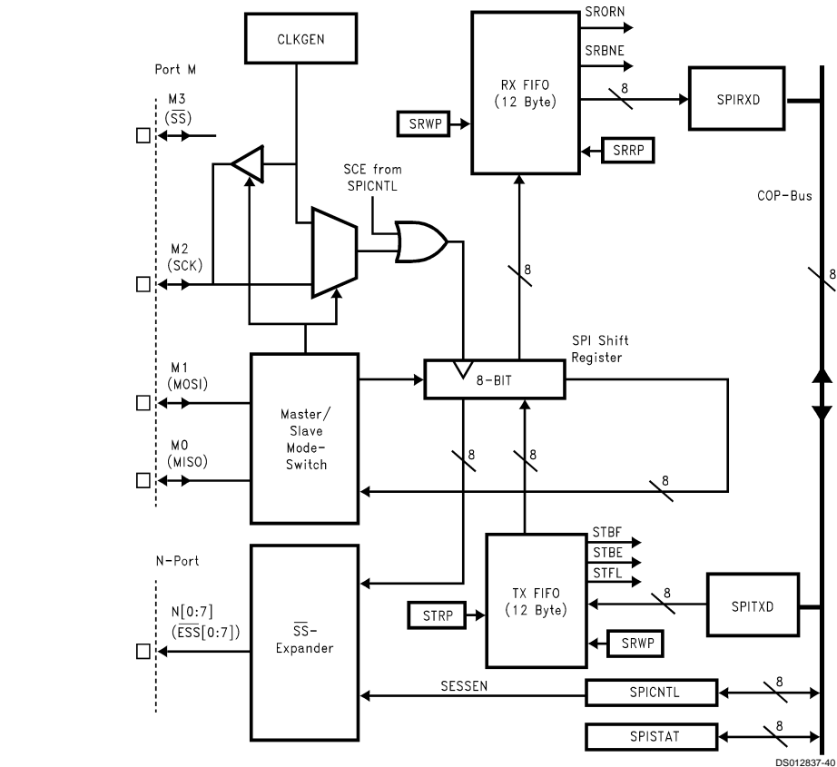
FIGURE 38. SPI Block Diagram
