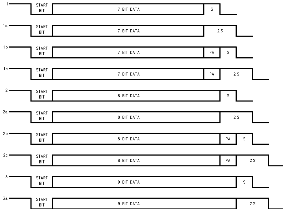
FIGURE 13. Framing Formats
