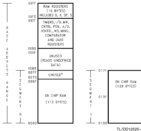
FIGURE 5. RAM Organization
