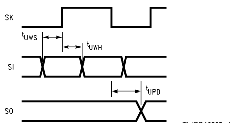
FIGURE 3. MICROWIRE/PLUS Timing
