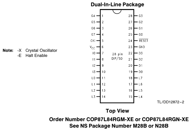
FIGURE 2. Connection Diagrams
