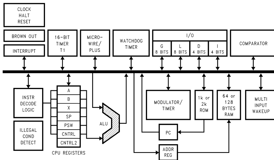
FIGURE 1. Block Diagram
