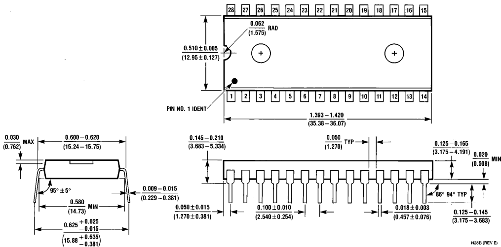
Molded Dual-In-Line Package (N) Order Number COP884EG-XXX/N NS Package Number N28B
