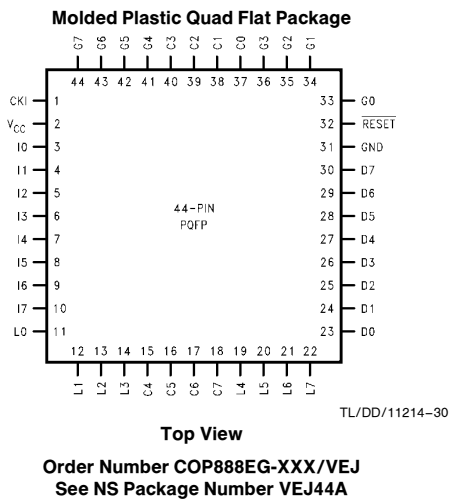
FIGURE 2a. Connection Diagrams
