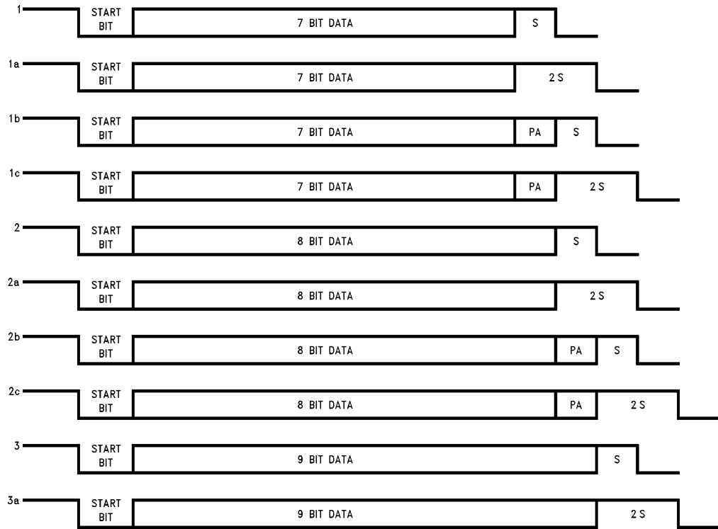
FIGURE 12. Framing Formats
