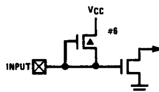
e. Input with Load
