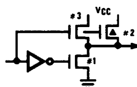
c. Push-Pull Output
