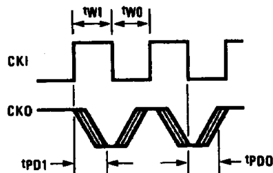
FIGURE 3b. CKO Output Timing
