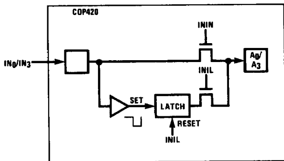
FIGURE 12. IN 0 /IN 3 Latches
