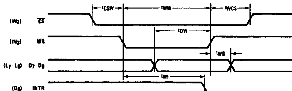
FIGURE 5. MICROBUS Write Operation Timing
