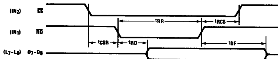
FIGURE 4. MICROBUS Read Operation Timing
