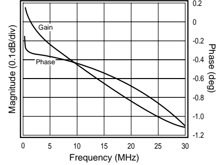
Frequency Response vs. V_o ( A_v = -1 )
