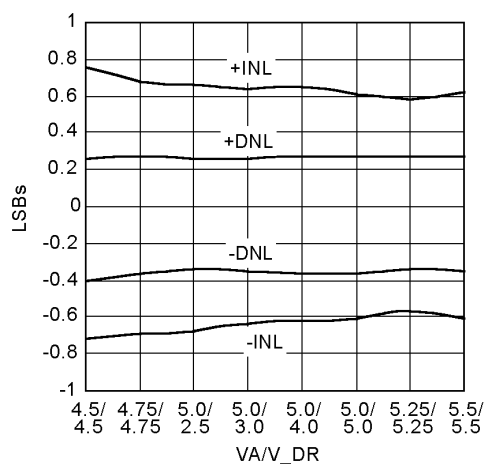
INL &amp; DNL vs Supply Voltage
