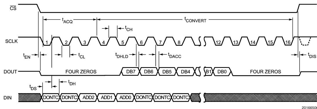
FIGURE 2. ADC088S102 Serial Timing Diagram
