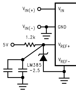
External Reference 2.5V Full-Scale (Standard Application)
