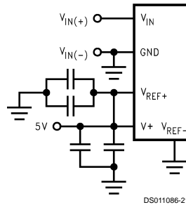
Power Supply as Reference
