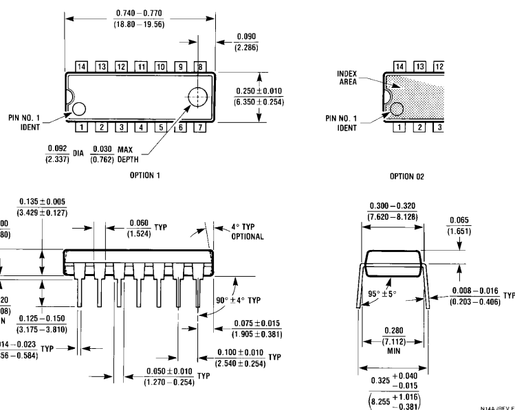
14-Lead Molded Dual-In-Line Package (N) Order Number DM7402N NS Package Number N14A
