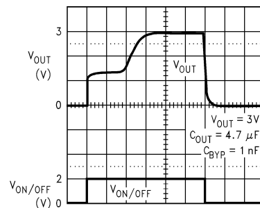
Turn-ON Waveform
